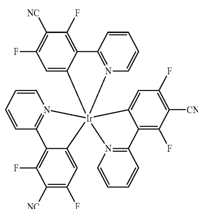
FCNIr
