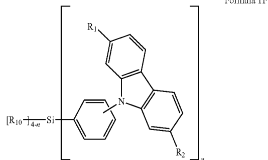
Formula 1F
