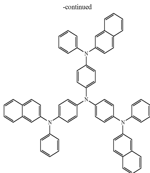
2-TNATA
