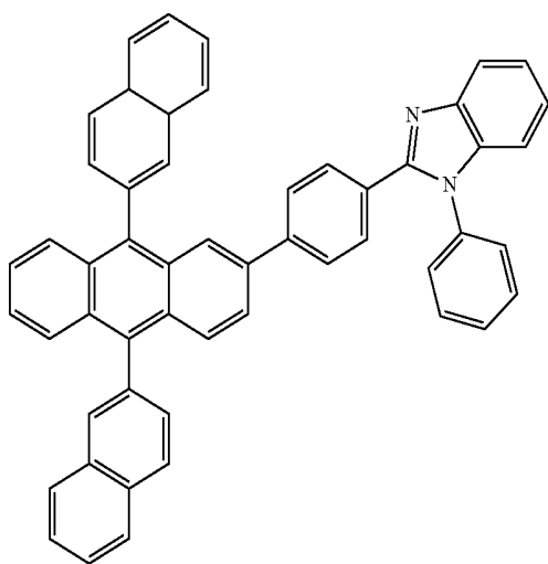
Compound 202
