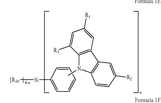
Formula 1F
