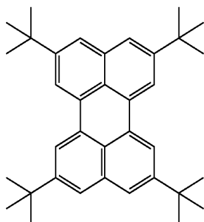
TBPc
