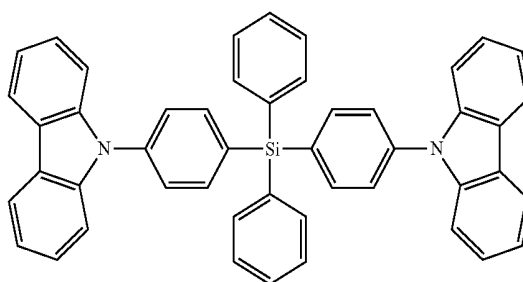
Compound A
