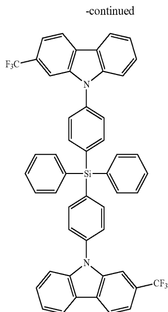
Compound 2
