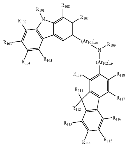
Formula 300
