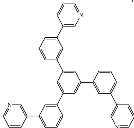
TmPyPB
